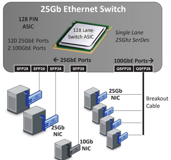
Figure 3. Proposed 25GbE Deployment Maximizes Bandwidth/Pin
